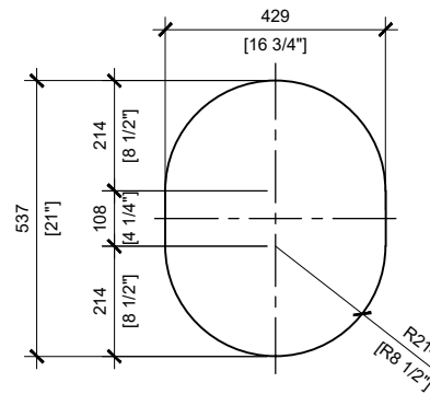
DETAIL 1 TOILET RISER OPENING (TYP.) SCALE: 1/16
