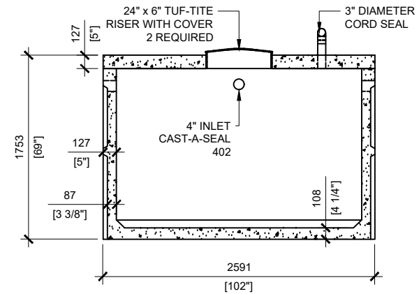
SECTION B SCALE:1/50
