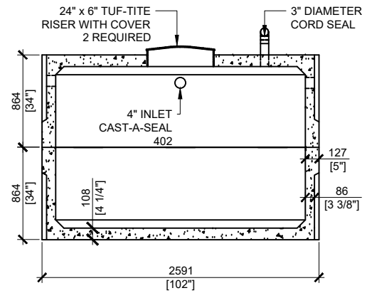
SECTION B SCALE:1/50
