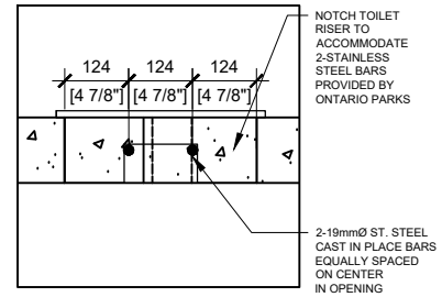
DETAIL 2: TOILET UNIT SECTION SCALE: 1/16
