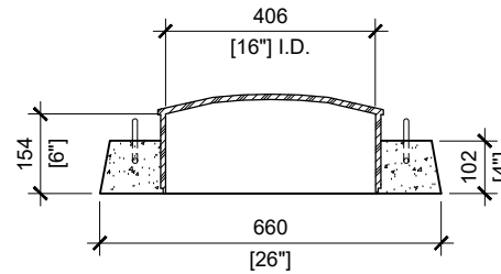
CROSS SECTION SCALE:1/16
