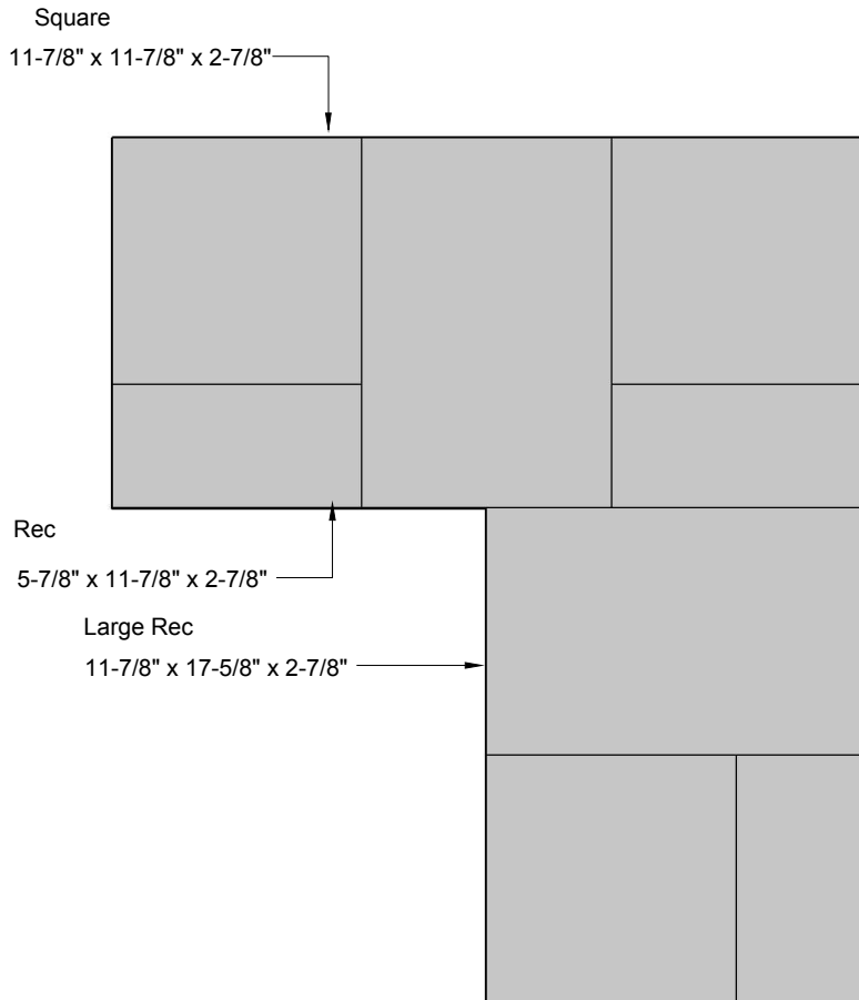
TYPICAL PATTERN BANFF
