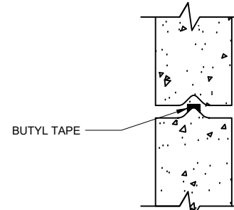
TONGUE & GROOVE JOINT SCALE: 1/8
