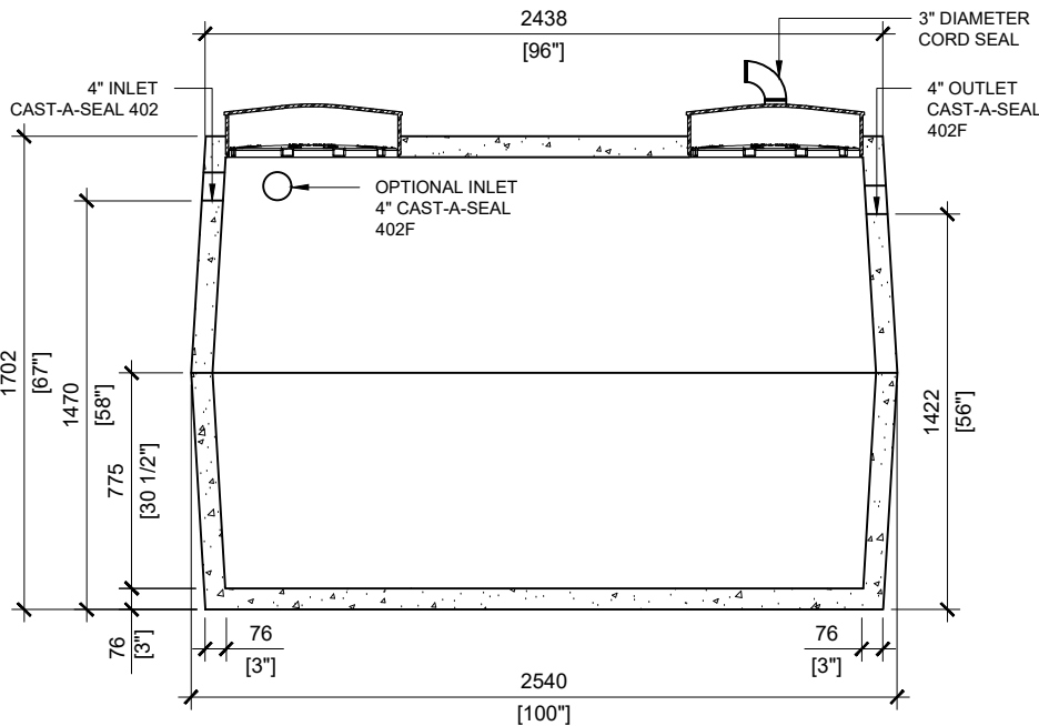
SECTION A SCALE:1/30
