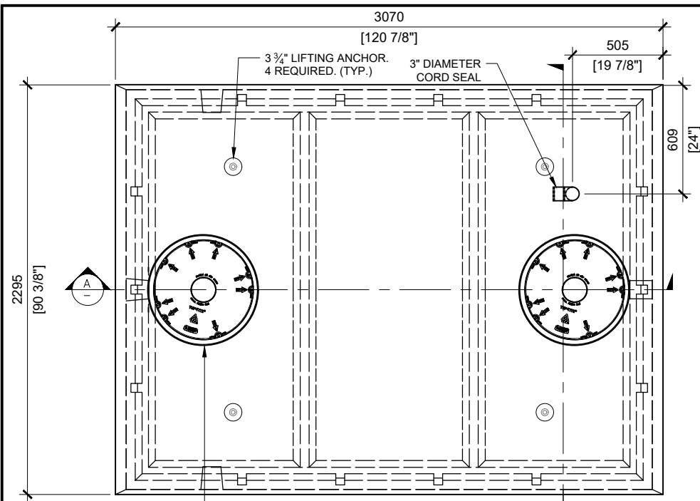
TOP VIEW SCALE: 1/30 3070 [120 7/8\"/>
