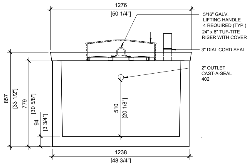
SIDE VIEW SCALE: 1/20
