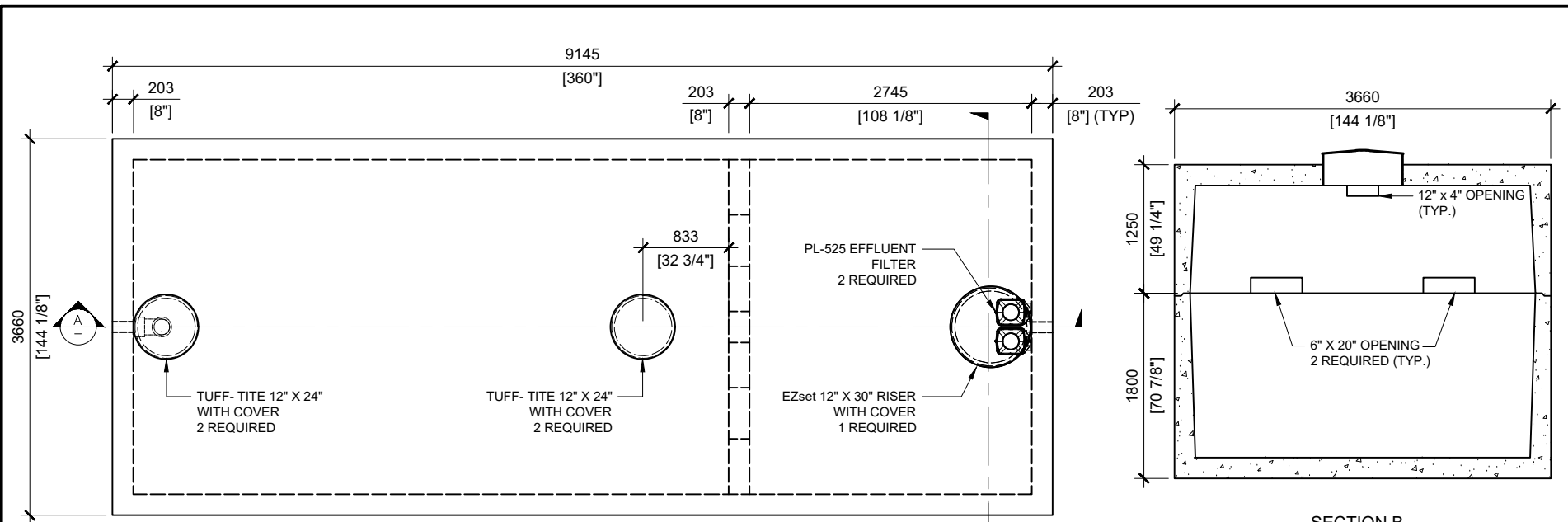
TOP VIEW SCALE:1/30
