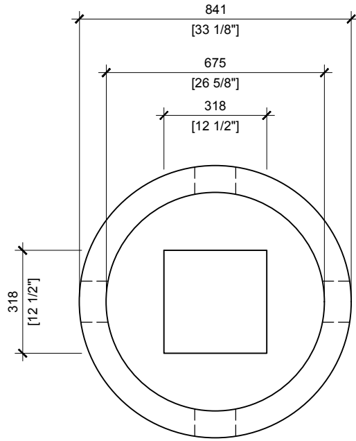
TOP VIEW SCALE: 1/16
