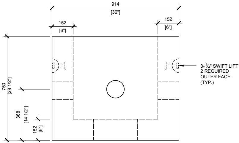
FRONT VIEW SCALE: 1/16
