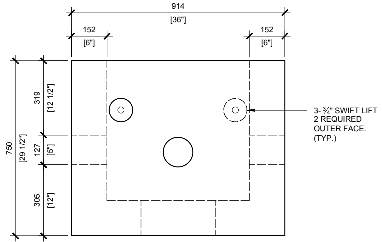
RIGHT VIEW SCALE: 1/16
