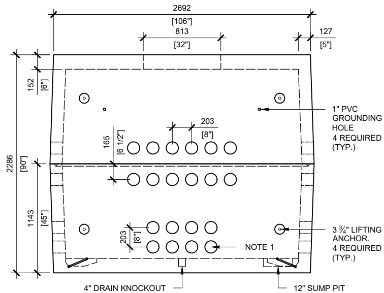
FRONT VIEW SCALE:1/40
