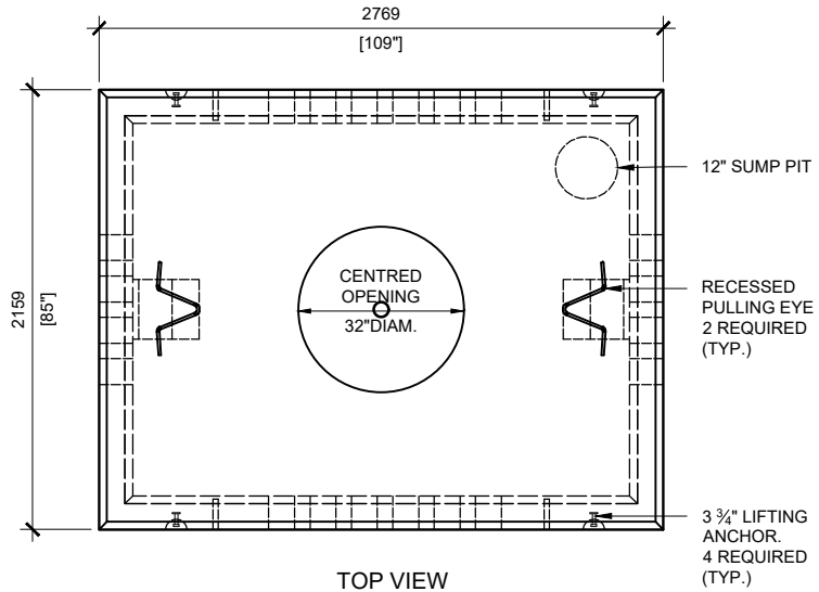
TOP VIEW SCALE:1/40
