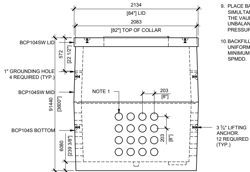
RIGHT VIEW SCALE:1/40
