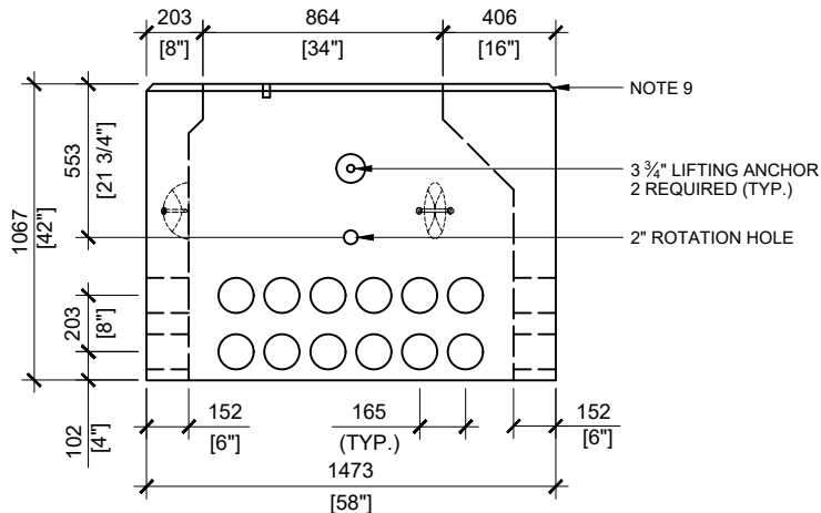
FRONT VIEW SCALE:1/30
