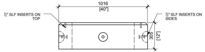
RIGHT VIEW SCALE:1/20
