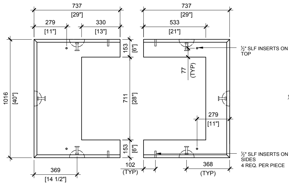
TOP VIEW SCALE:1/20
