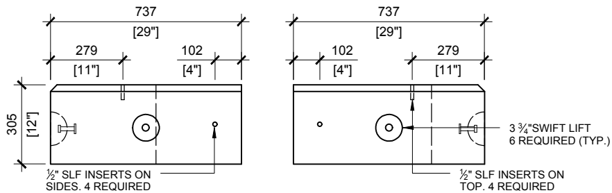
FRONT VIEW SCALE:1/20
