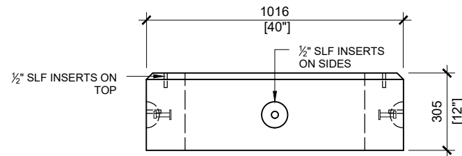
RIGHT VIEW SCALE:1/20
