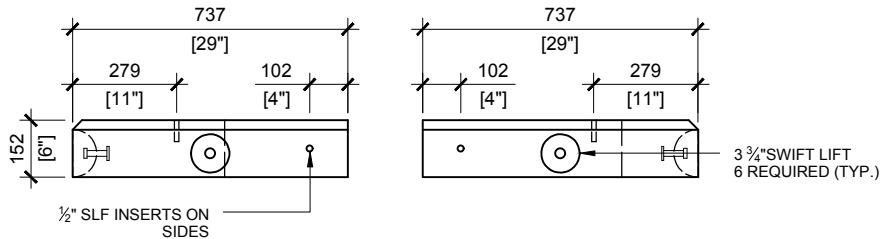
FRONT VIEW SCALE:1/20
