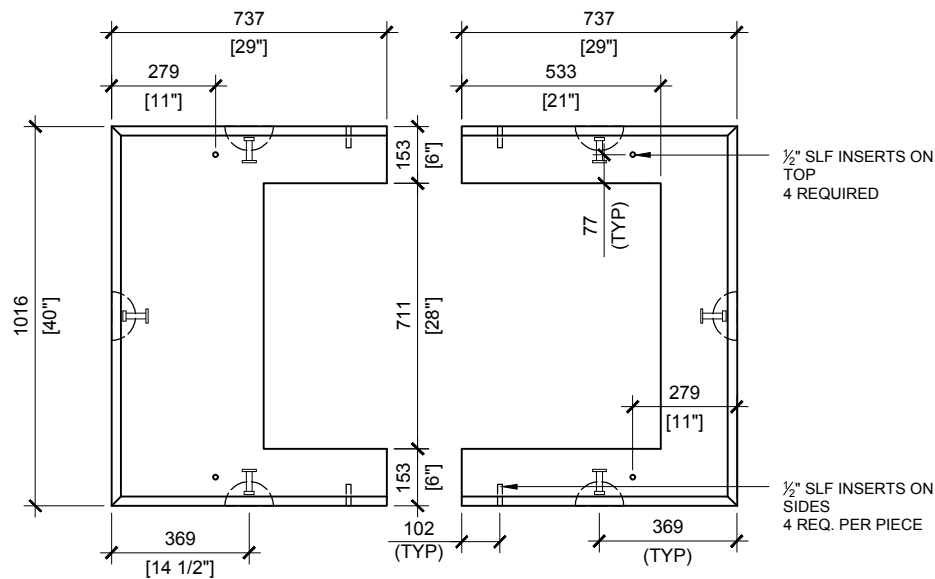
TOP VIEW SCALE:1/20
