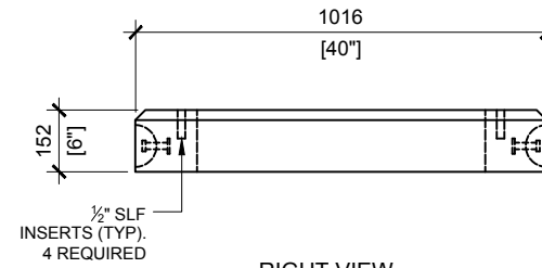
RIGHT VIEW SCALE:1/20
