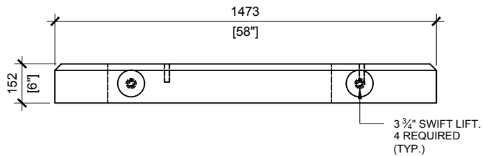
FRONT VIEW SCALE:1/20
