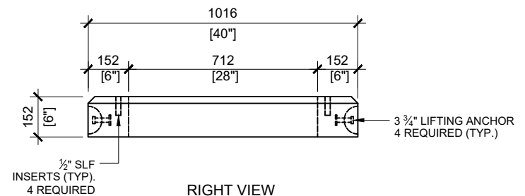
RIGHT VIEW SCALE:1/20
