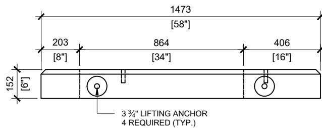
FRONT VIEW SCALE:1/20
