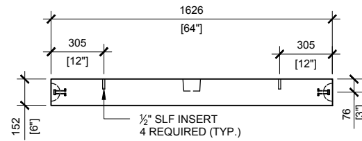
RIGHT VIEW SCALE:1/30
