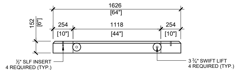
RIGHT VIEW SCALE:1/30
