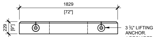
BCP114T9H20 FRONT VIEW SCALE:1/40
