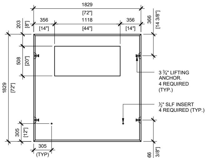
BCP114T6 TOP VIEW SCALE: 1/40
