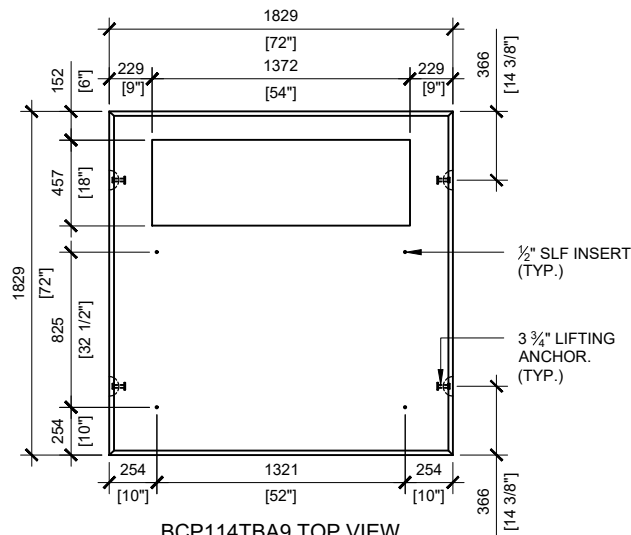
BCP114TBA9 TOP VIEW SCALE:1/40
