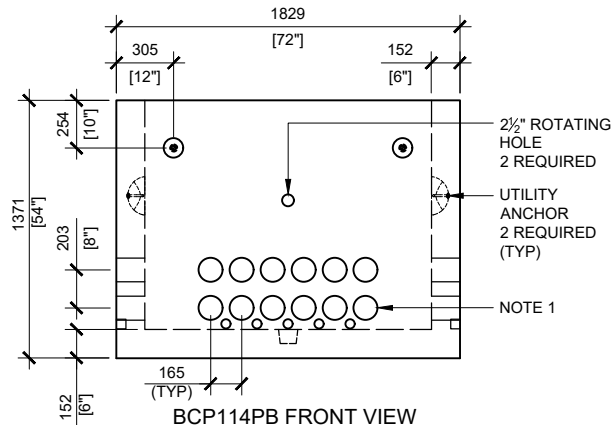
BCP114PB FRONT VIEW SCALE:1/40
