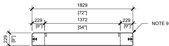
BCP114TBA9 FRONT VIEW SCALE:1/40
