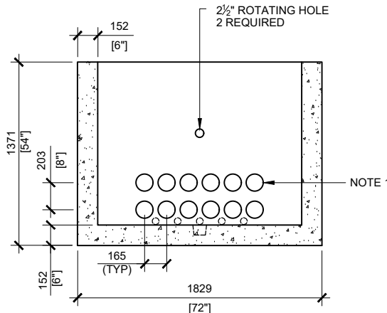
SECTION A SCALE:1/40
