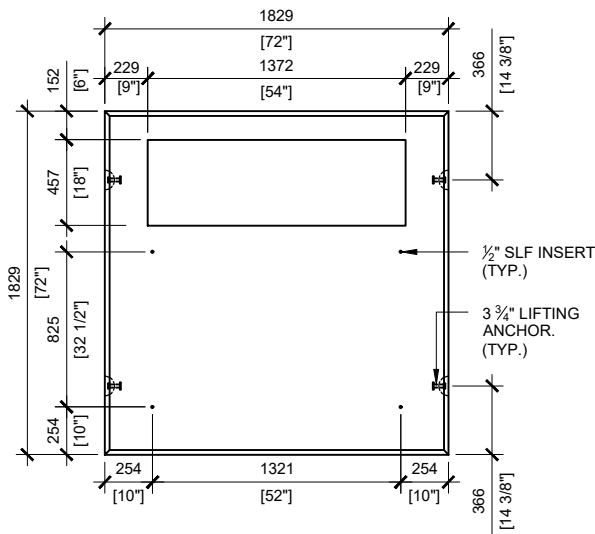
BCP114TBA9 TOP VIEW SCALE:1/40
