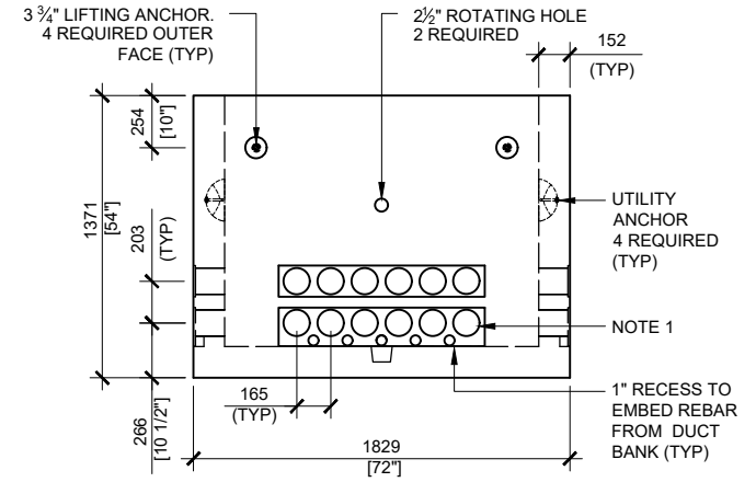
BCP114PB FRONT VIEW SCALE:1/40
