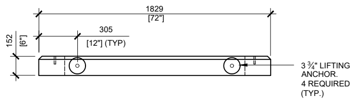
FRONT VIEW SCALE: 1/30
