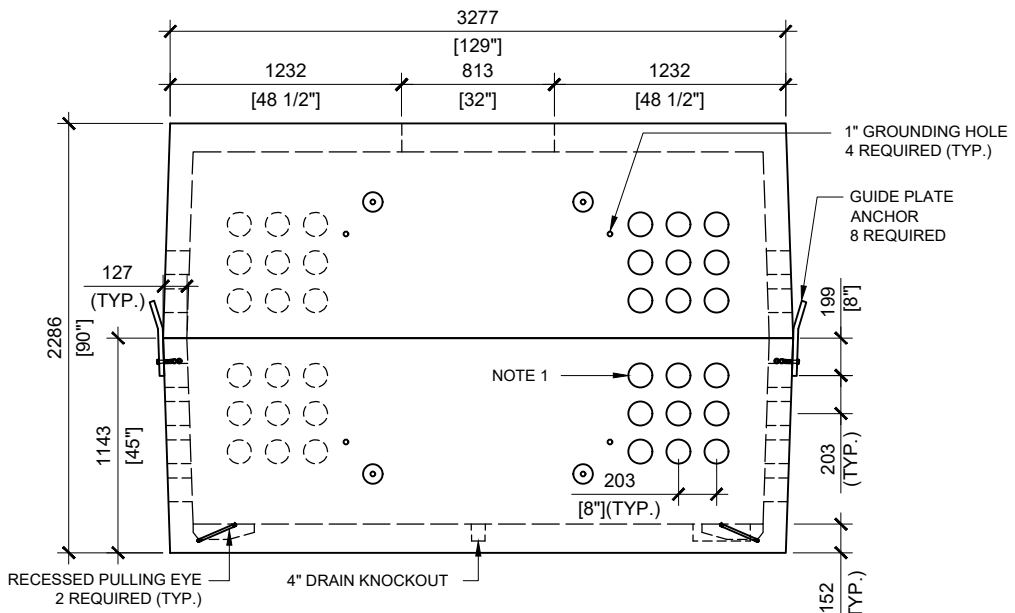
FRONT VIEW SCALE: 1/40
