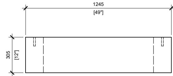
RIGHT VIEW SCALE: 1/40
