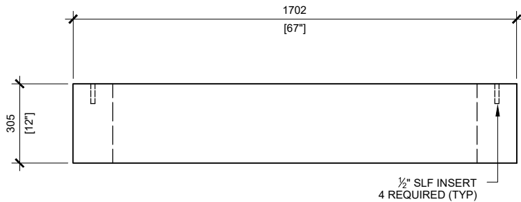
FRONT VIEW SCALE: 1/40
