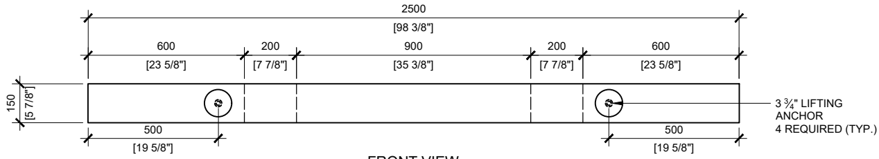
FRONT VIEW SCALE: 1/20
