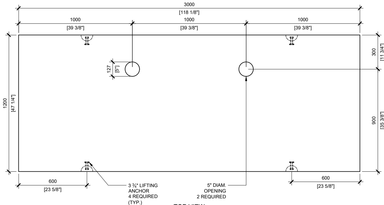
TOP VIEW SCALE:1/20
