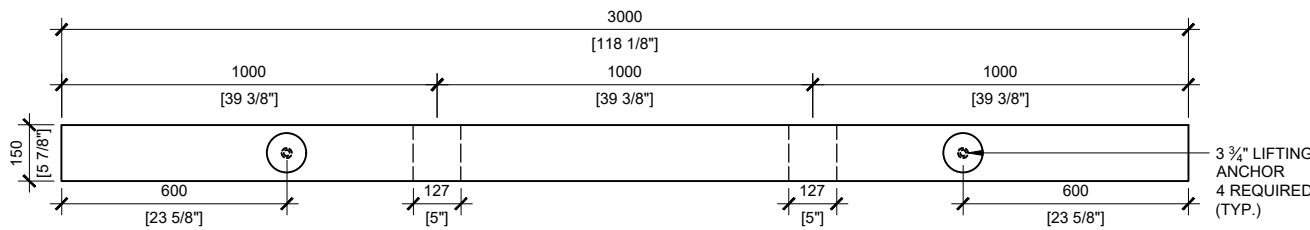
FRONT VIEW SCALE:1/20
