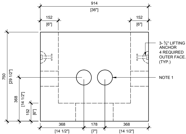
FRONT VIEW SCALE: 1/16
