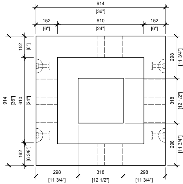
TOP VIEW SCALE: 1/16
