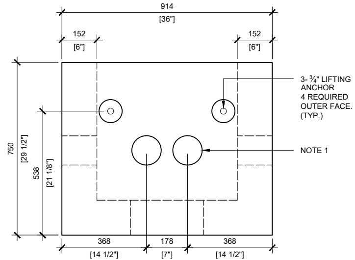
RIGHT VIEW SCALE: 1/16
