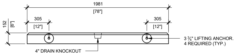
FRONT VIEW SCALE:1/30
