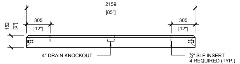
RIGHT VIEW SCALE:1/30
