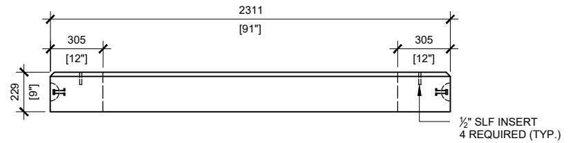
RIGHT VIEW SCALE:1/30
