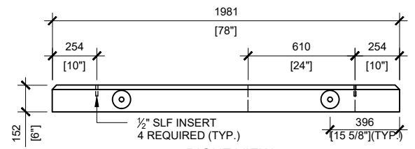
RIGHT VIEW SCALE:1/30
