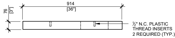
BCP36P LID FRONT VIEW SCALE:1/20
