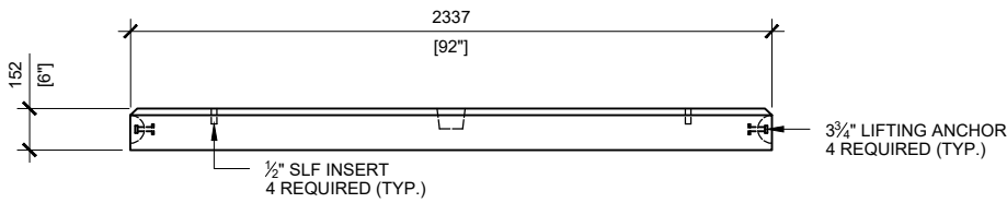
FRONT VIEW SCALE:1/30
