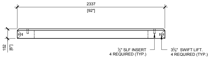
FRONT VIEW SCALE:1/30
