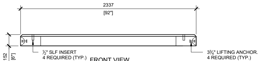
FRONT VIEW SCALE:1/30
