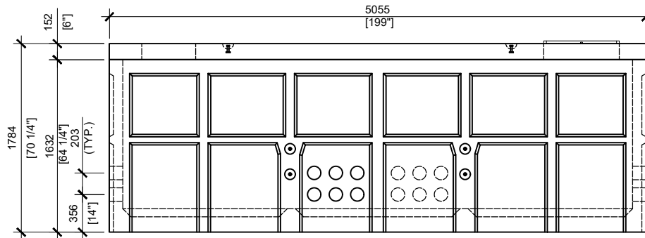
FRONT VIEW SCALE: 1/50
