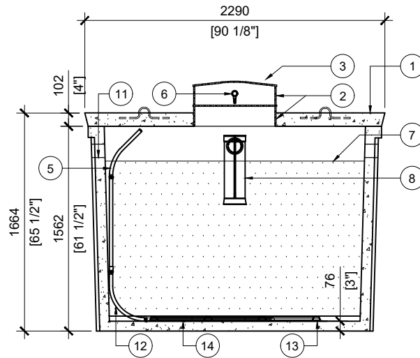
SECTION B SCALE:1/30
