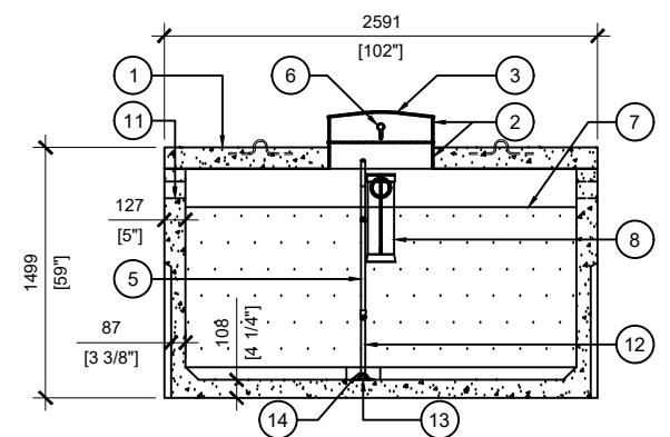
SECTION B SCALE:1/50
