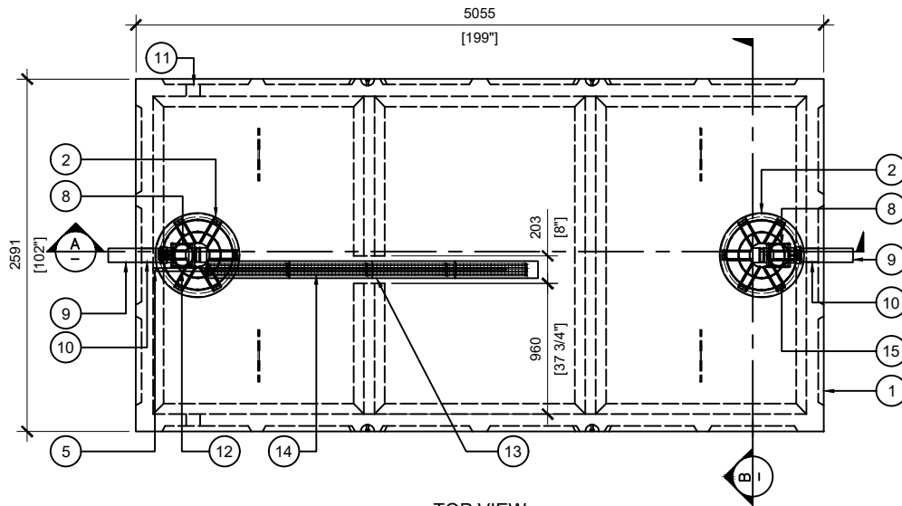
TOP VIEW SCALE:1/50
