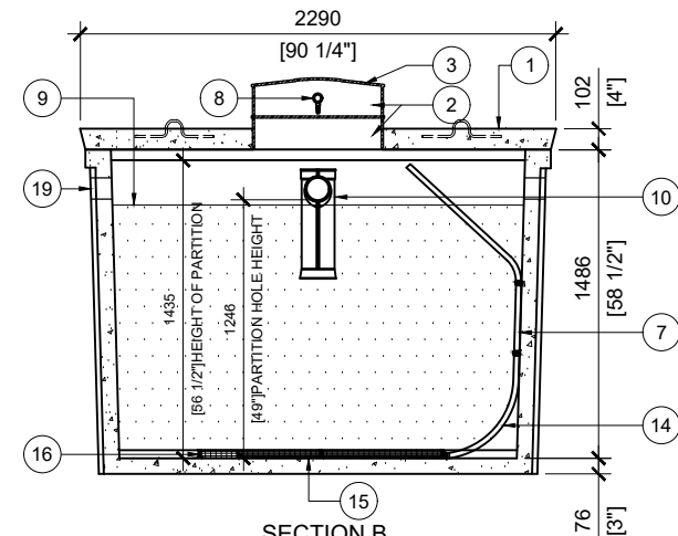
SECTION B SCALE:1/40
