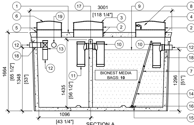
SECTION A SCALE:1/40
