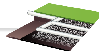
POLISHING FIELD TREATED WATER DISCHARGE
