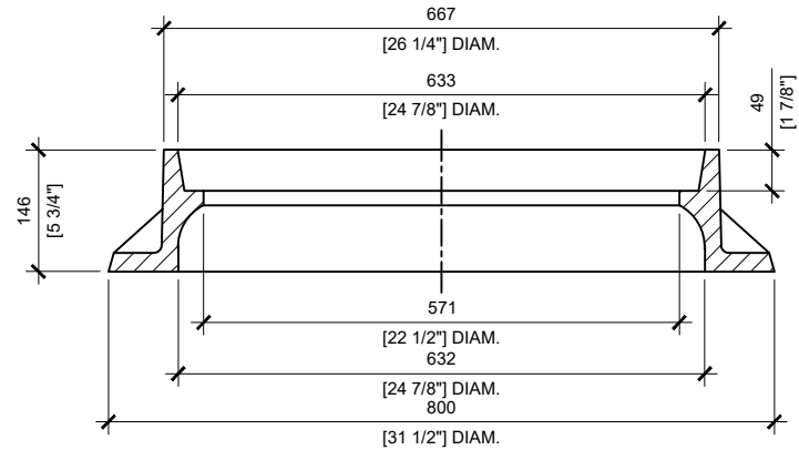
ACCESS FRAME TOP VIEW SCALE:1/10
