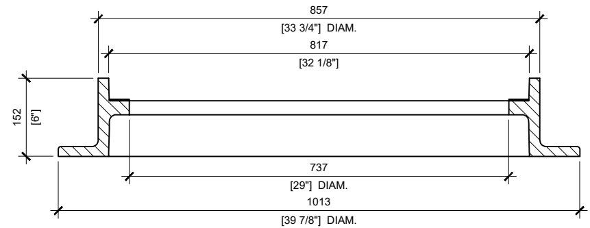
ACCESS FRAME TOP VIEW SCALE:1/10
