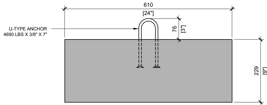
FRONT VIEW SCALE: 1/8
