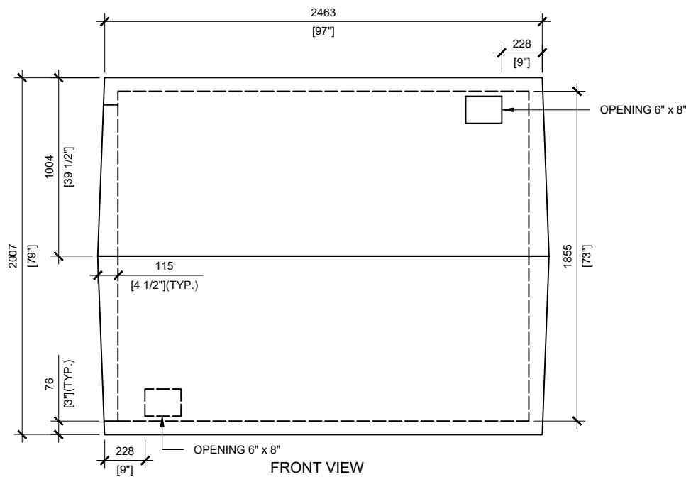
FRONT VIEW SCALE: 1/30
